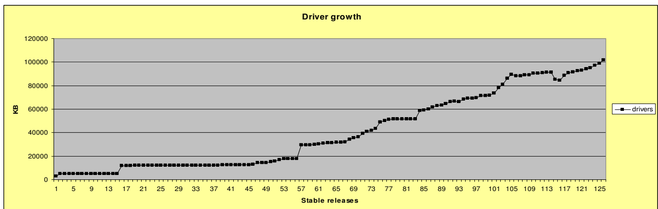
Figure 6B. Linux kernel sub-system.
