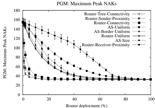
Fig. 23. PGM back-off timer interval sensitivity: PGM Maximum Peak NAKs with 4 * worst RTT as the back-off timer interval
