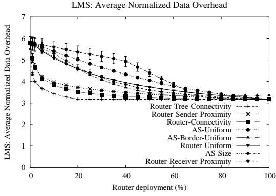
Fig. 8. LMS Average Normalized Data Overhead
