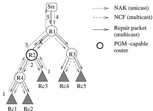
Fig. 2. PGM example
