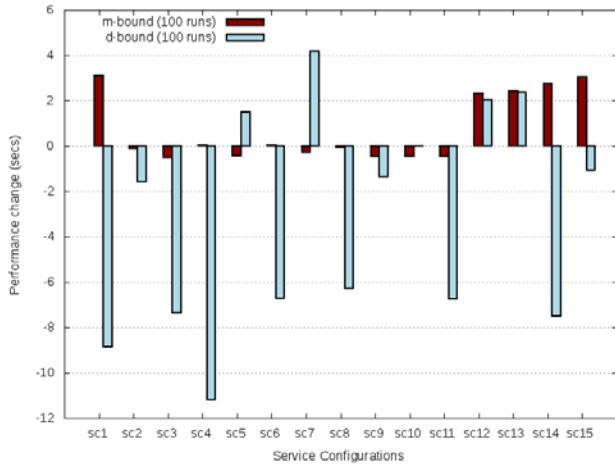
Figure 4. 10GB VM Performance Changes (seconds)
