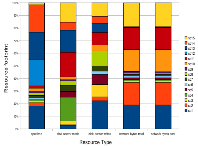
Figure 1. Resource Utilization Variation of Component Deployments
