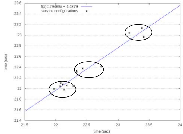
Figure 2. 4GB “m-bound” regression plot
