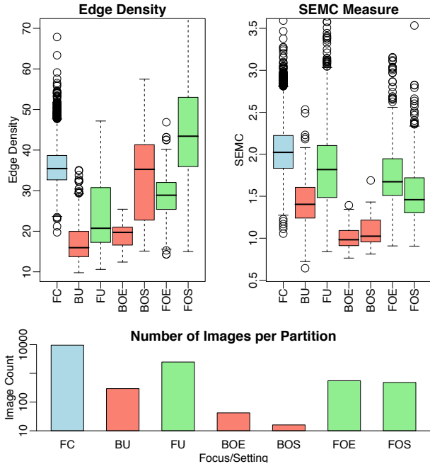
Figure 2. Comparison of edge density and SEMC focus measures. Red indicates partitions manually annotated as blurry while the green partitions were judged to be in focus. Blue indicates controlled lighting images, which are essentially all in focus. The bottom plot shows the number of images in each partition. Images annotated as blurry account for 10% of the uncontrolled and outdoor images.
