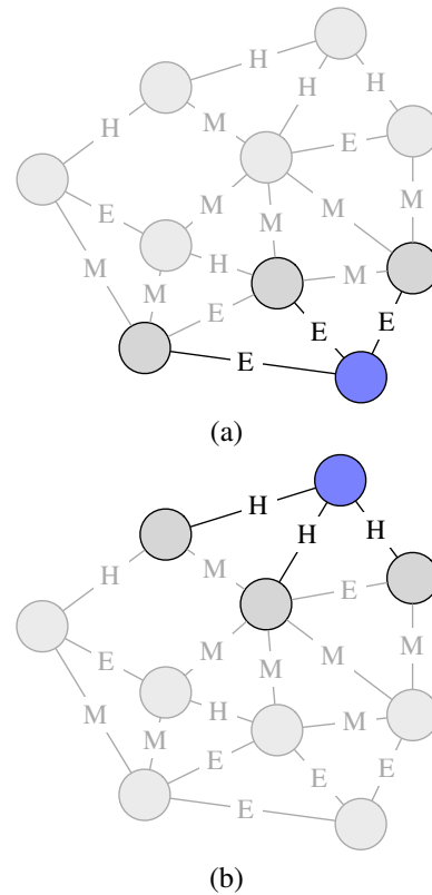
Fig. 2. Examples illustrating subgraph patterns associated with images that are: a) always easy to recognize and, b) always hard to recognize.
