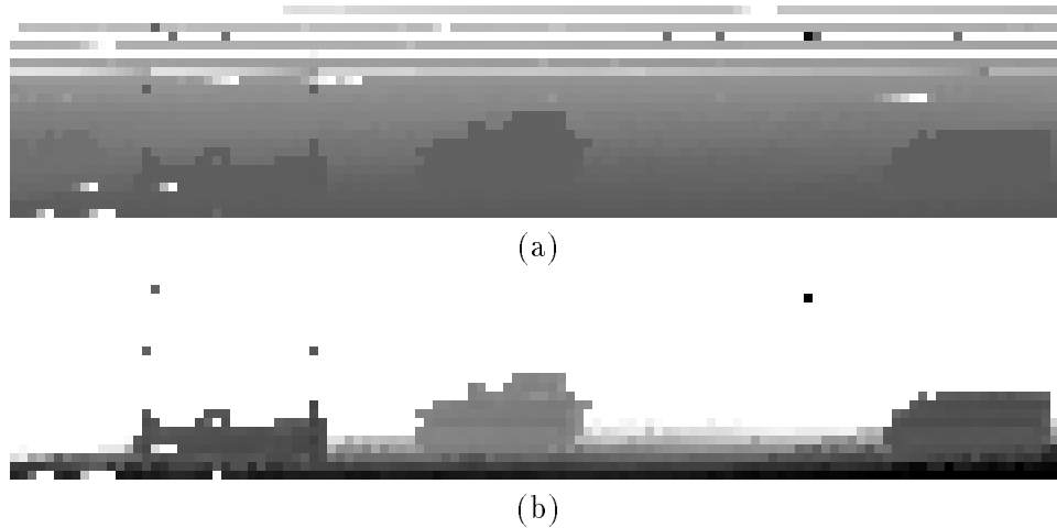
Figure 15: LADAR image nov11010l showing M113-901. a) full 100 to 1,000 foot range, b) range highlighted about vehicle.
