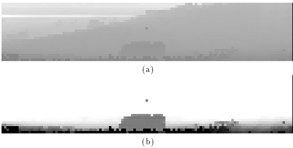
Figure 18: LADAR image nov31055l showing M60. a) full 100 to 1,000 foot range, b) range highlighted about vehicle.
