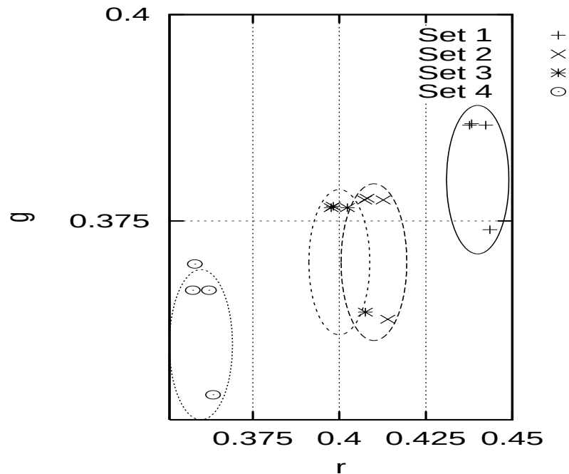
Figure 6.5. Estimates of the apparent color of the concrete slabs under four sets (results labeled “Set 1”, “Set 2”, and so on, corresponding to respective entries in Table 6.4) of conditions—represented by corresponding confidence intervals—under a sample set of conditions. The figure shows that 14 observations out of 16 lie within the respective confidence intervals.
