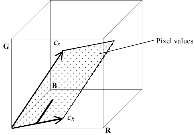
Figure 5.1. The Dichromatic Model [43][80] describes reflectance in RGB space as a skewed “L”-shaped cluster within a parallelogram that represents the dichromatic plane.
