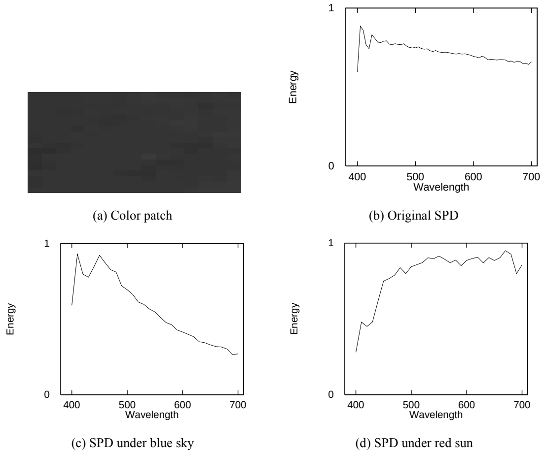
Figure 2.7. The Munsell blue (number 10Bv9c1) patch (a) with the SPD representing its albedo (b), and the SPD's under (c) blue sky, and (d) red sun.
