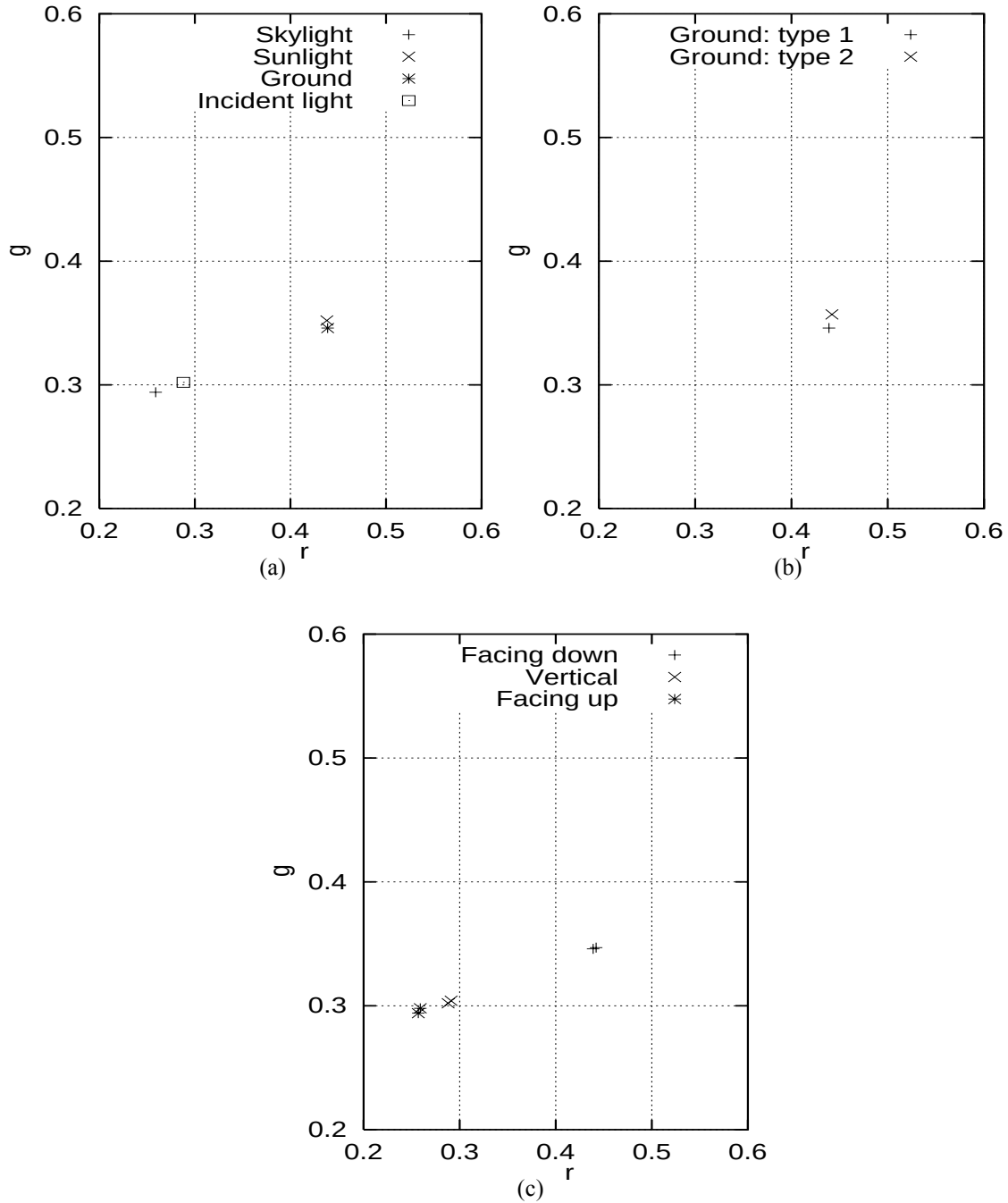
Figure 4.5. Samples of daylight color obtained from color images: (a) the color of skylight (“Skylight”), sunlight (“Sunlight”), the effective incident light (“Incident”) measured using the white surface, along with a direct measurement of the “average” ground color (“Ground”); (b) direct samples of the “average” ground color (averaged over 30 \times 30 regions), measured from two different locations; (c) samples of the white surface at different orientations (facing down, vertical, and facing up).
