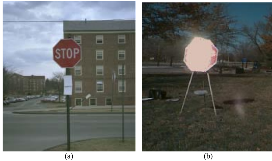
Figure 1.3. Images of a specular “Stop” sign at two different orientations: (a) facing away from the sun; (b) facing the sun.
