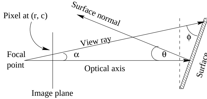
Figure 6.1. Viewing geometry for image pixels: The viewing angle( \phi ) for a pixel at position [r,c] equals (90 + \alpha - \theta) , where \theta is the angle between the optical axis and the surface normal, and \alpha is the angle of the viewing ray at pixel [r,c] , which is determined the field-of-view of the camera.
