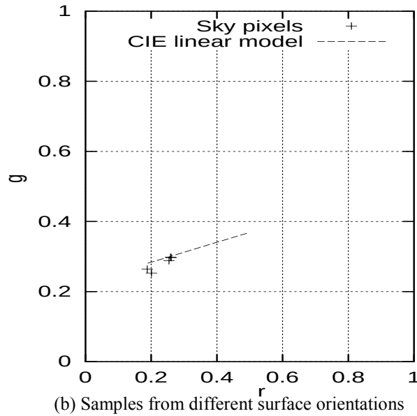
Figure 4.4. Samples of direct skylight color obtained from different portions of the sky: (a) experimental setup demonstrating how direct samples of the sky at different angles (with the camera facing away from the sun) were collected—samples were collected with the angle between the camera axis and the ground plane ( \theta ) at 5^\circ , 15^\circ , 30^\circ , 45^\circ and 85^\circ ; (b) the samples plotted against the linearized CIE model. The data demonstrates that different portions of the sky can exhibit different colors.
