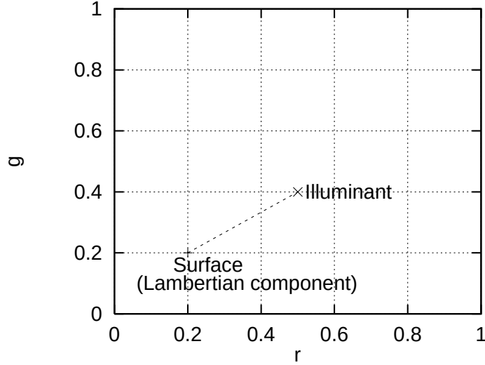
Figure 5.2. The Dichromatic Reflectance model in normalized color space. The apparent color of the surface is a point on the line between the points representing the colors of the illuminant and the Lambertian component of the surface under that illuminant.
