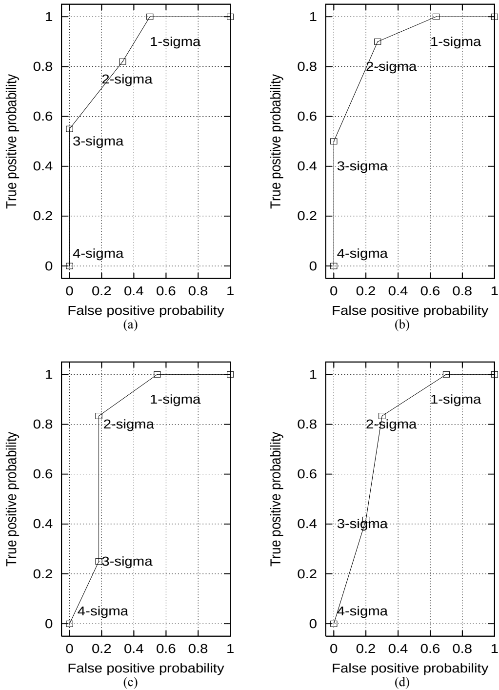
Figure 6.8. ROC curves for the (a) "Stop" sign, (b) "No Parking" sign, (c) concrete slab, and (d) road asphalt. The curves plot the probability of a true positive against the probability of a false positive for confidence intervals of \sigma , 2\sigma , 3\sigma and 4\sigma . Based on the above curves, a 2\sigma confidence interval was chosen for all four surfaces.
