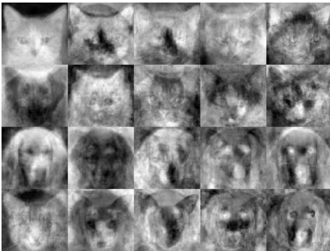
Fig. 6. First five eigenvalues for each of the clusters in Fig. 4.
