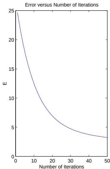
Figure 4: The value of E versus the number of iterations.
