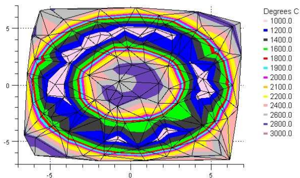
Contour Plot of the Heat Distribution of a Plasma Torch
