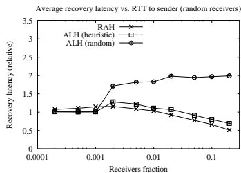
Fig. 21. RAH and ALH topology sensitivity (Random graph): average data recovery latency.
