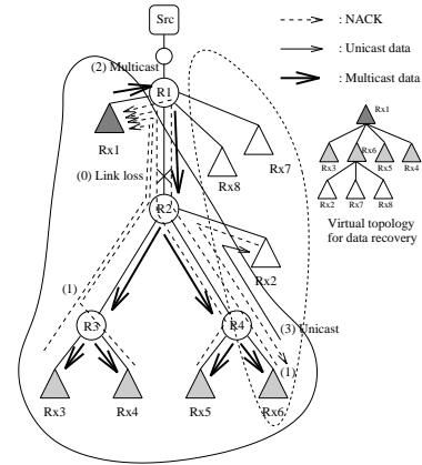
Fig. 2. ALH example: sub-optimal hierarchy organization
