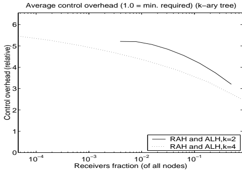
Fig. 8. Average control overhead (same for RAH and ALH).
