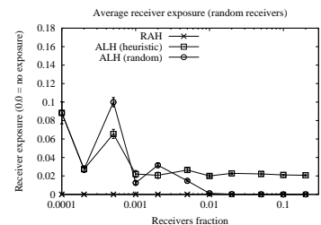
Fig. 12. RAH and ALH (Internet core): average receiver exposure.
