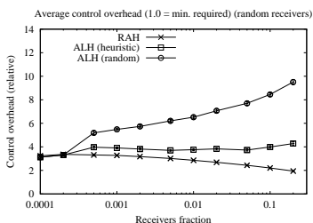
Fig. 14. RAH and ALH (Internet core): average control overhead.
