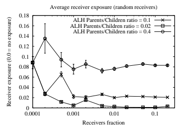
Fig. 16. ALH: receiver exposure sensitivity to hierarchy organization.
