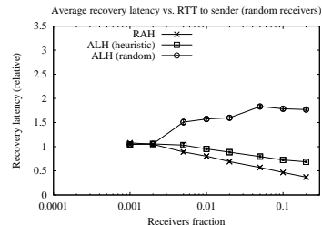
Fig. 20. RAH and ALH topology sensitivity (Mbone): average data recovery latency.
