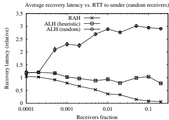
Fig. 22. RAH and ALH topology sensitivity (Mesh): average data recovery latency.
