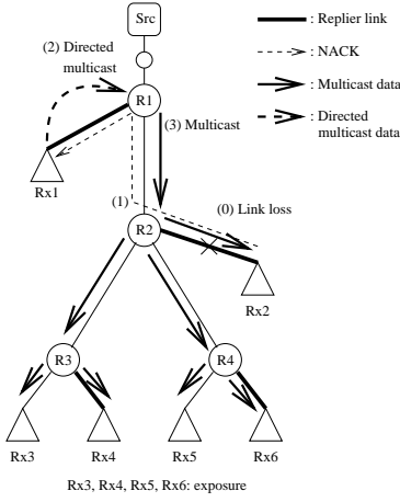
Fig. 4. LMS vanilla example: data loss by replier only and exposure to other receivers
