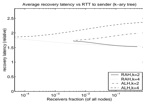
Fig. 10. RAH and ALH: average data recovery latency.
