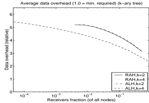
Fig. 9. RAH and ALH: average data overhead.
