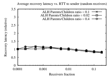
Fig. 15. ALH: data recovery latency sensitivity to hierarchy organization.
