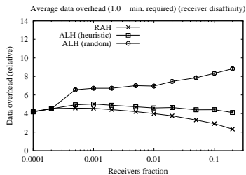
Fig. 25. RAH and ALH (Internet core, receiver disaffinity): average data overhead.
