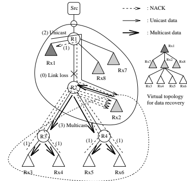
Fig. 1. ALH example: optimal hierarchy organization
