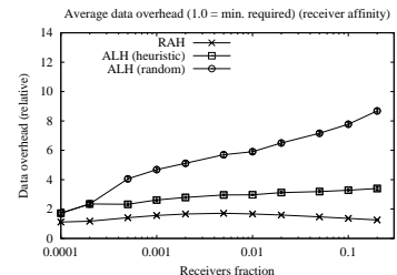
Fig. 24. RAH and ALH (Internet core, receiver affinity): average data overhead.
