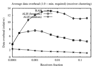
Fig. 26. RAH and ALH (Internet core, receiver clustering): average data overhead.
