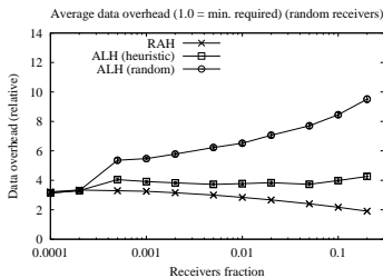
Fig. 13. RAH and ALH (Internet core): average data overhead.
