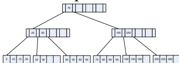
B + -tree for instructor file ( n = 5 )
