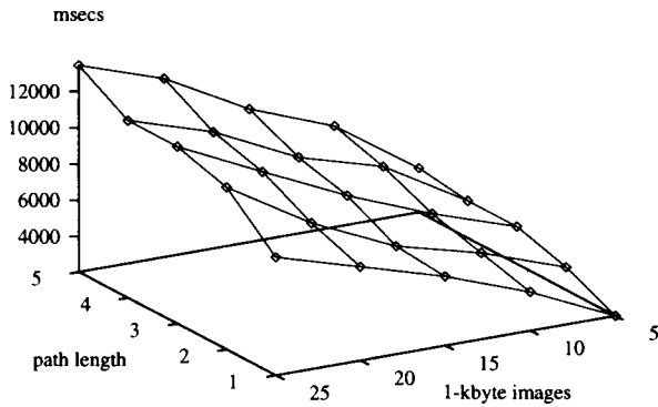
Fig. 5. Response latency (msecs) as a function of path length and number of embedded images.
