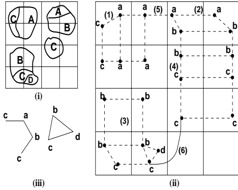
Figure 4: Example of SPG construction (i) Synthetic image divided into cells (ii) Cells marked with nodes (peaks) contained in them. The intermediate graph is shown in broken lines (iii) SPG constructed from (ii)
