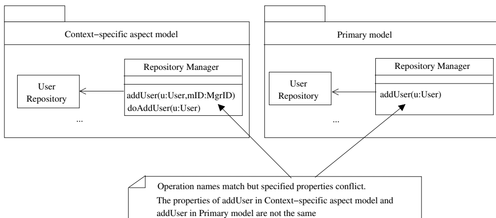
Fig. 4. Example of a Property Conflict
