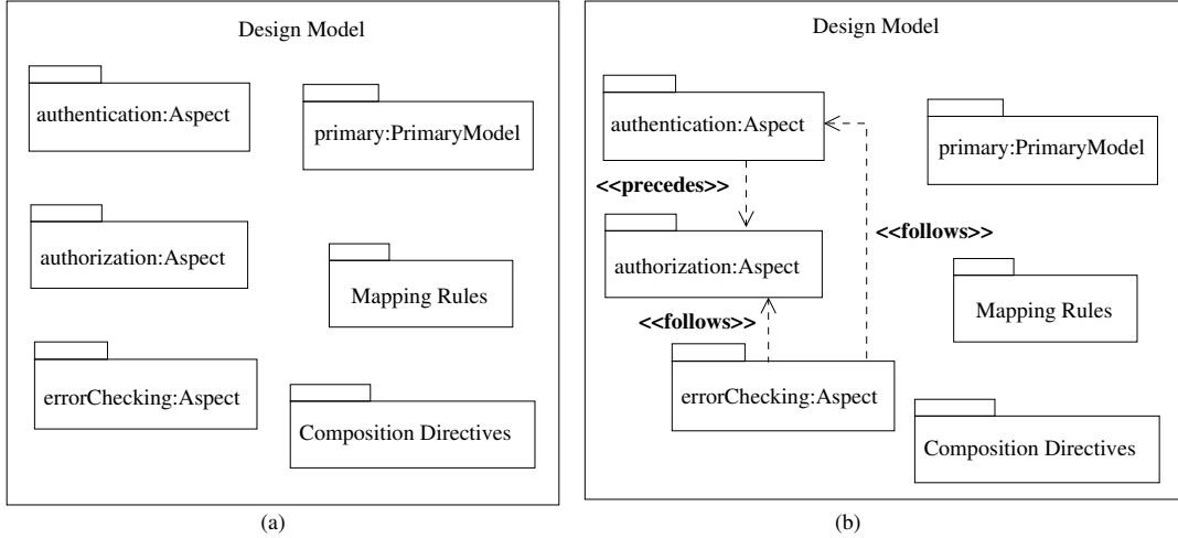
Fig. 11. Example 4. Specifying Weave Order
