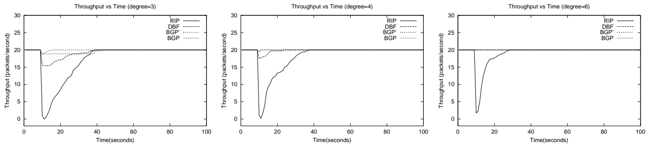
Figure 5. Instantaneous Throughput
