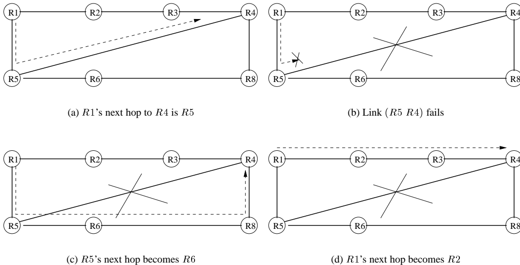
Figure 1. Packet Could still Be Delivered during Convergence
