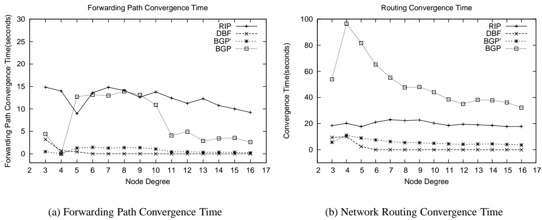
Figure 6. Forwarding Path Convergence Time and Routing Convergence Time
