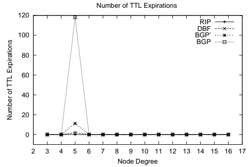
Figure 4. Number of TTL Expirations During Convergence
