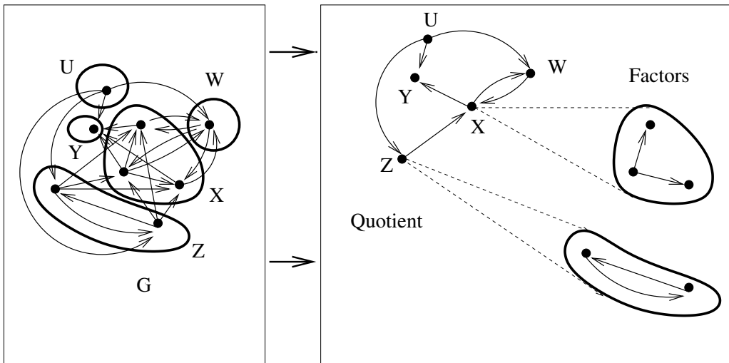
Figure 2: If A and B are disjoint modules, then if B contains a neighbor of a vertex in A , every member of B is a neighbor of every member of A . In this case, B is adjacent to A . A partition \mathcal{P} of G where each member of \mathcal{P} is a module defines a quotient graph , which describes the adjacencies among members of \mathcal{P} . The quotient, together with the subgraphs induced by the nontrivial members of \mathcal{P} , give a representation of G , since the edges of G can be recovered from them.
