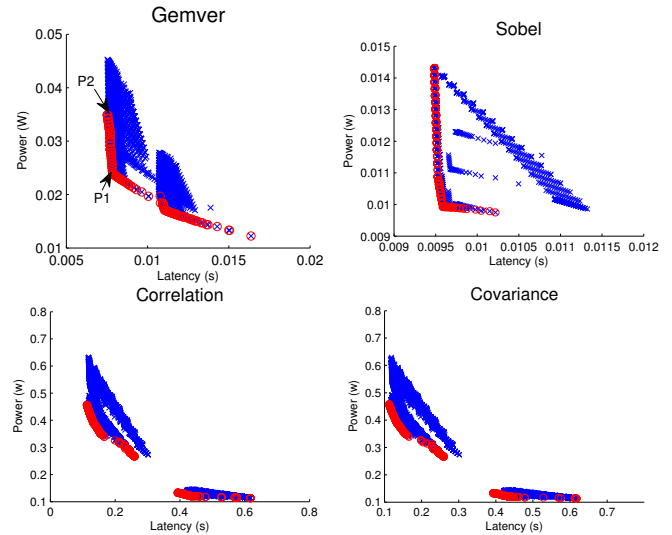
Fig. 7. Modeled design space and Pareto points
