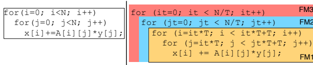
Fig. 3. Left: C/C++ code fragment isolated by PolyOpt. Right: tiled code and equivalent Function Modules generated. FM1 is a tile of size T \times T .
