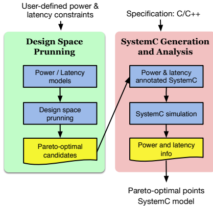
Fig. 6. Overview of the DSE framework
