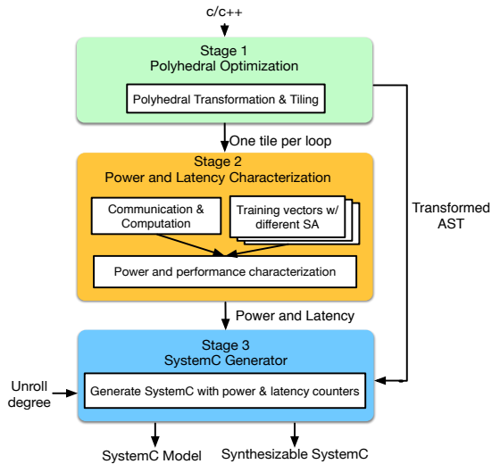
Fig. 1. SystemC generation and analysis framework
