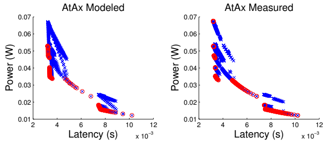
Fig. 5. Modeled design space and measured design space
