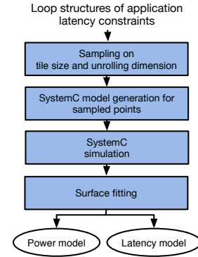
Fig. 4. Analytical power/latency modeling framework
