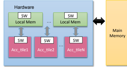
Fig. 2. Architecture of the generated accelerator
