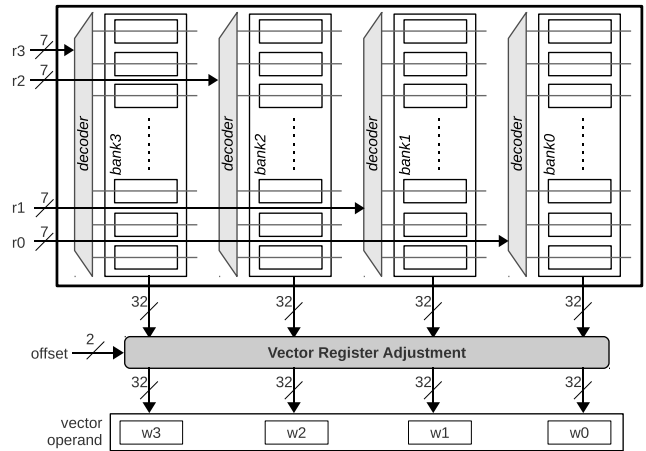
Figure 4. Read-port of a modified VRF including the VRA logic.
