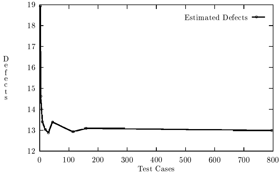
Figure 9: Estimated total defects with new approach (Vouk data set 3)
