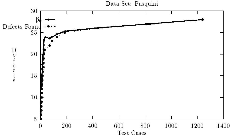
Figure 6: Estimated total defects using exponential model (Pasquini data)
