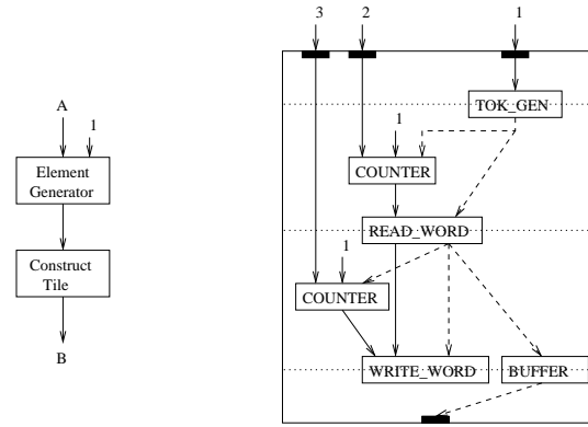
Figure 5. One-dimensional array copy in dataflow and AHA.
