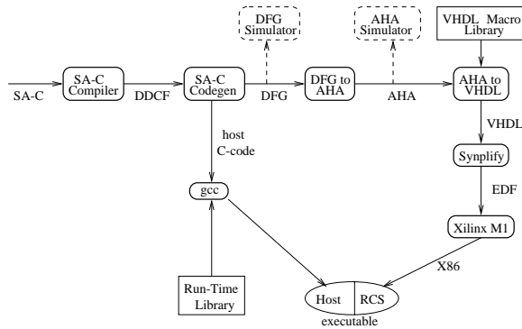
Figure 1. SA-C Compilation system.
